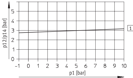
MFH-5/3...-3/8-S-B
